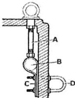
Stern Assembly
