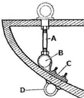
Bow Assembly
